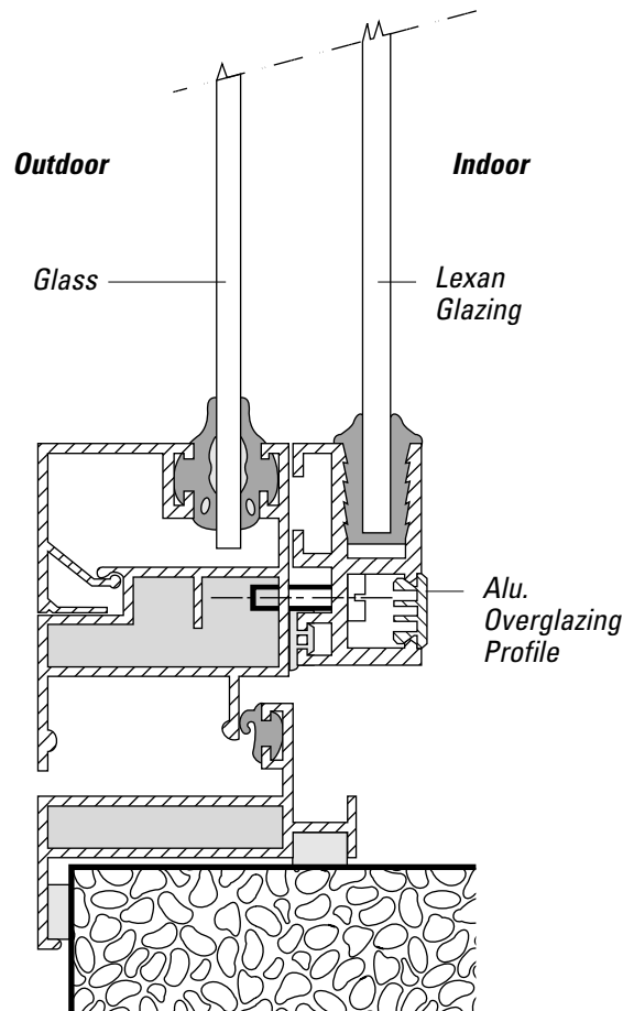
Fig. 23: Internal Overglazing
