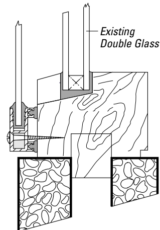
Fig. 24: External Overglazing
