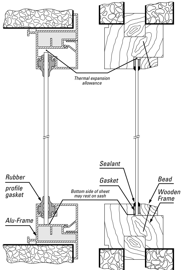
Dry glazing installation
