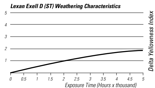
Fig. 8: Delta Yellowness Index (ASTM D1925)
