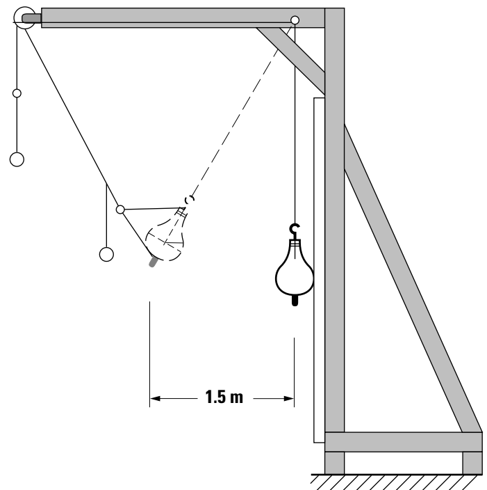
Fig. 5: Balcony Glazing Test DIN 52337 Hard/Soft Body Impact
