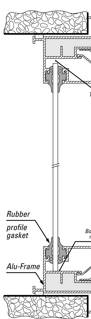
Dry glazing installation
